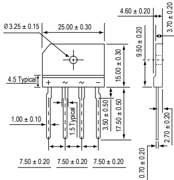
GBPC-W
