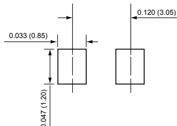
SOD-123 SOD-123 (Flat lead)
