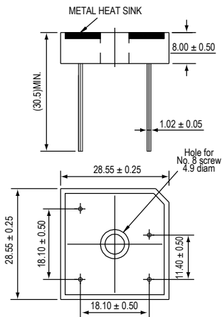
GBPC-W
