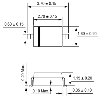
SOD-123
