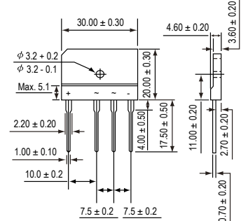
GBJ GBJ-LB
