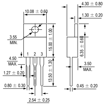
TO-220AB
