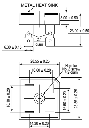
GBPC
