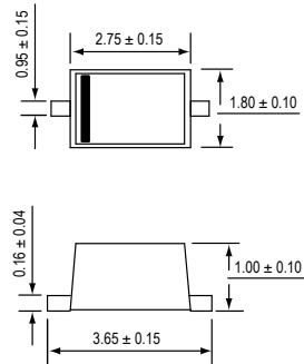
SOD-123 FL
